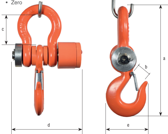
Dimensions (mm)
